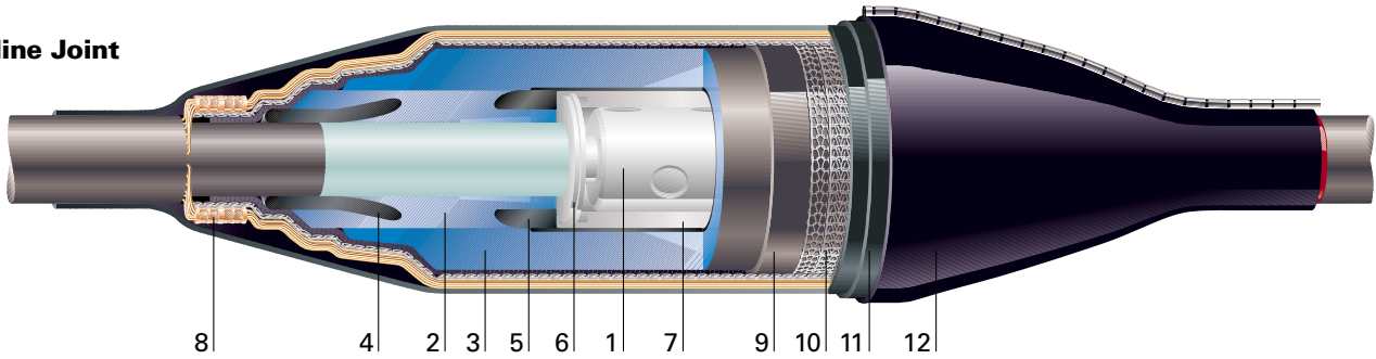
Shield-Break Joint
