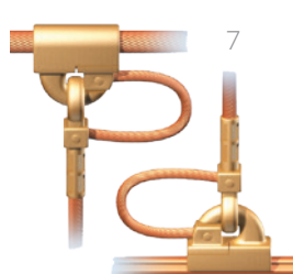
Catenary Dropper System
